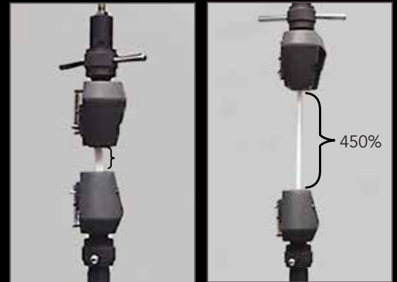
DEK-650 Flexible Membrane achieves 450% elongation as performed by ASTM D638.
