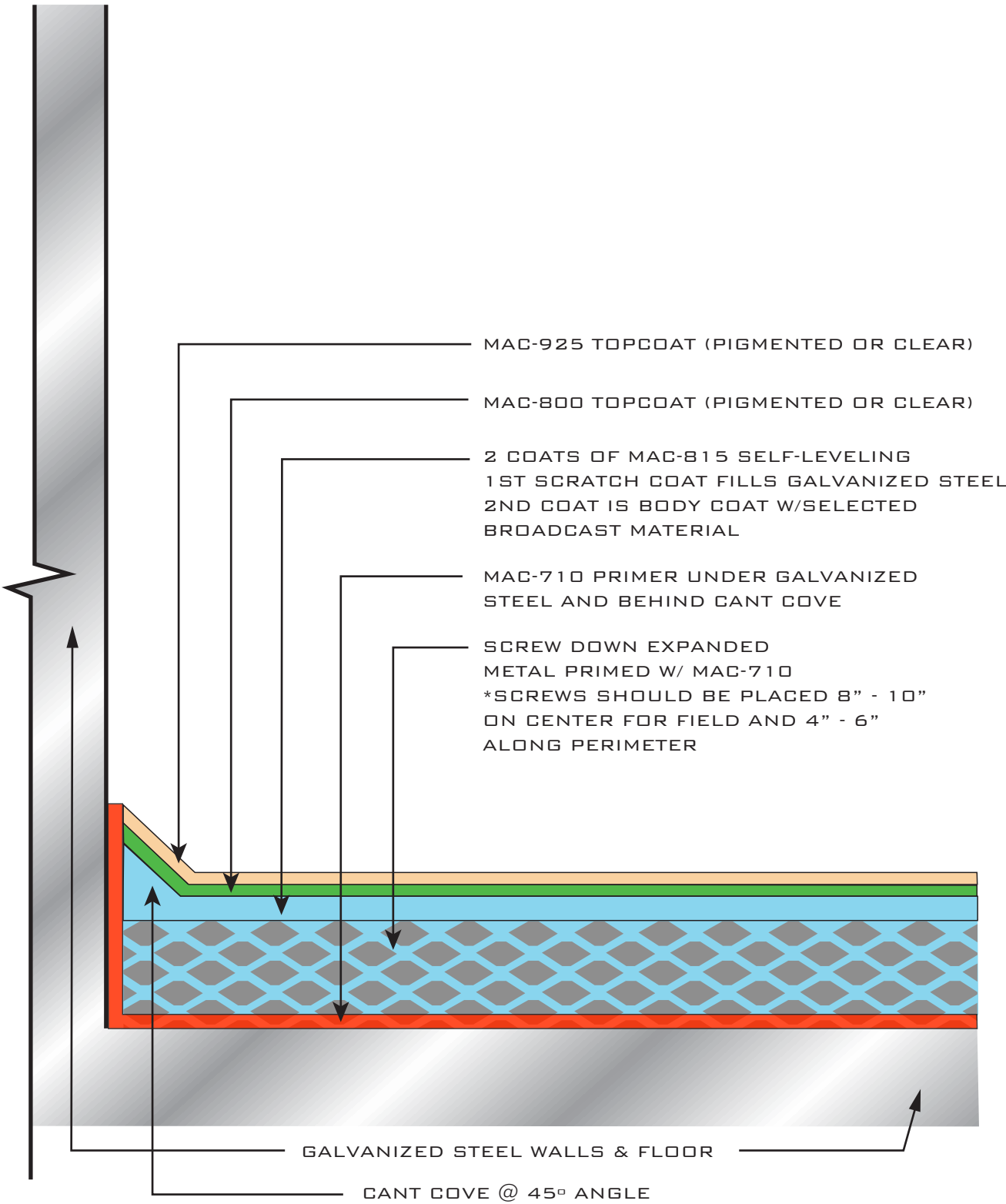
FIGURE F.3 COOLER/FREEZER FLOORING SYSTEM NOT TO SCALE
