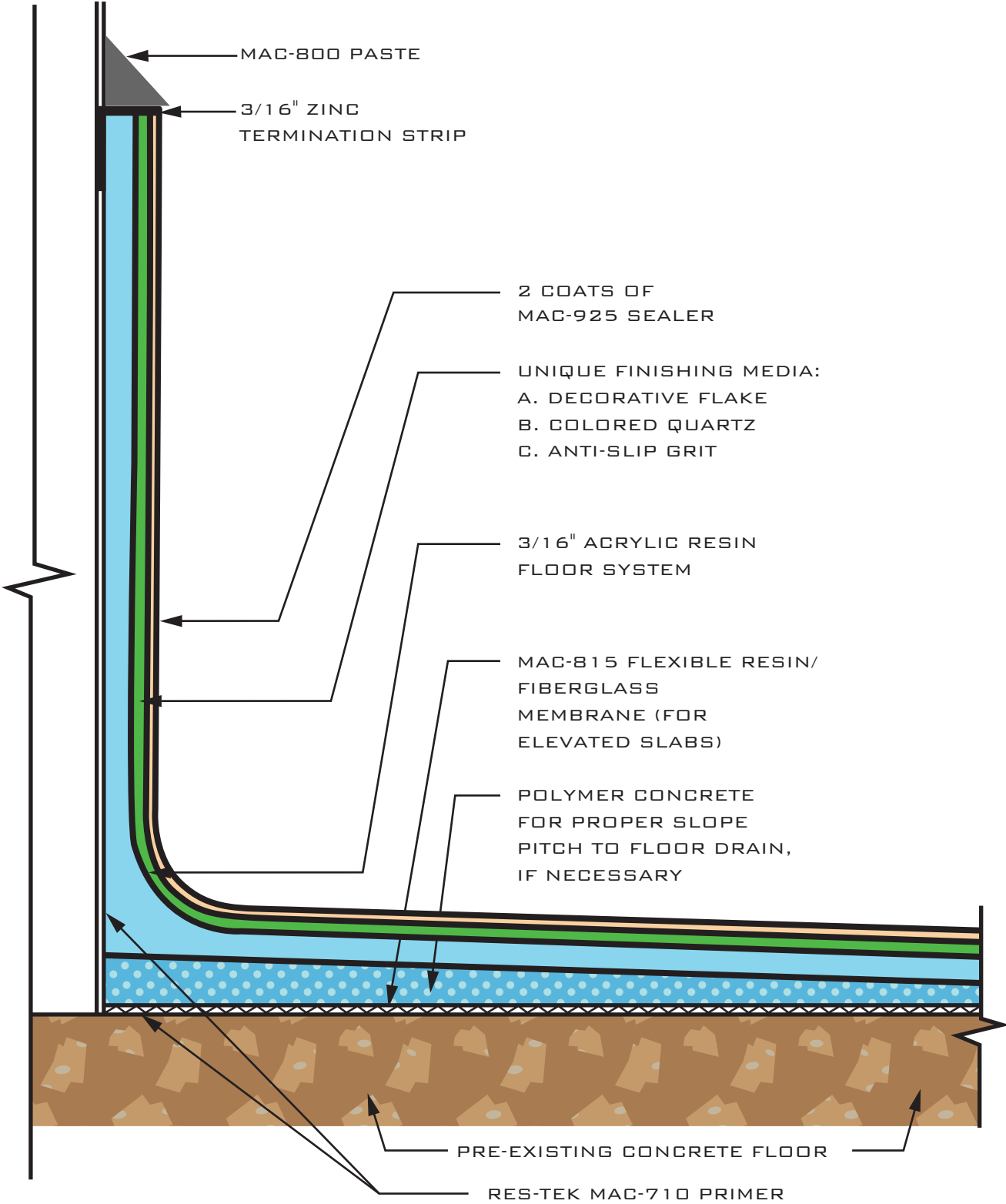
FIGURE A.2 ACRYLIC MEMBRANE FLOOR SYSTEM WITH CANT
