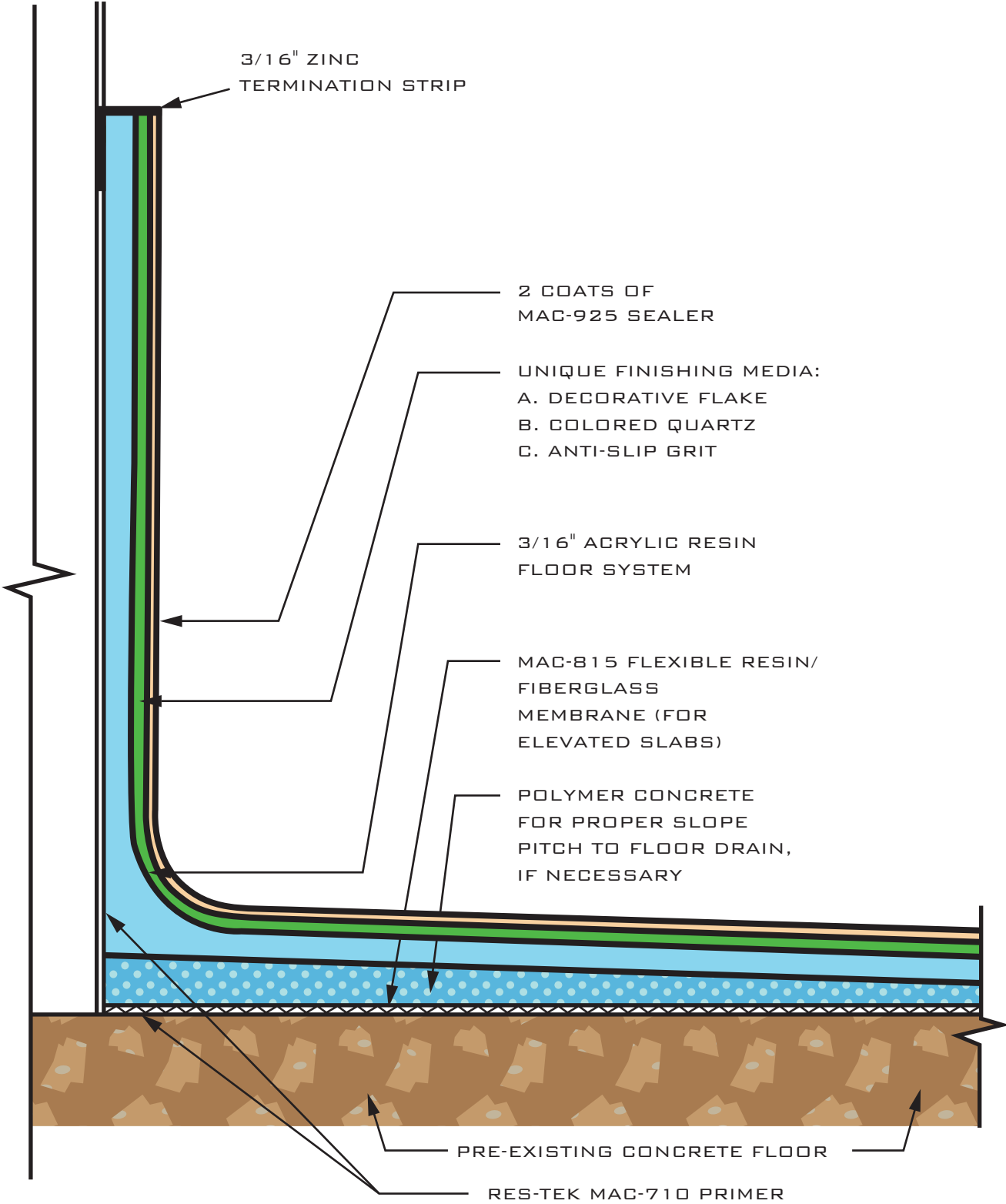
FIGURE A.1 ACRYLIC MEMBRANE FLOOR SYSTEM NOT TO SCALE
