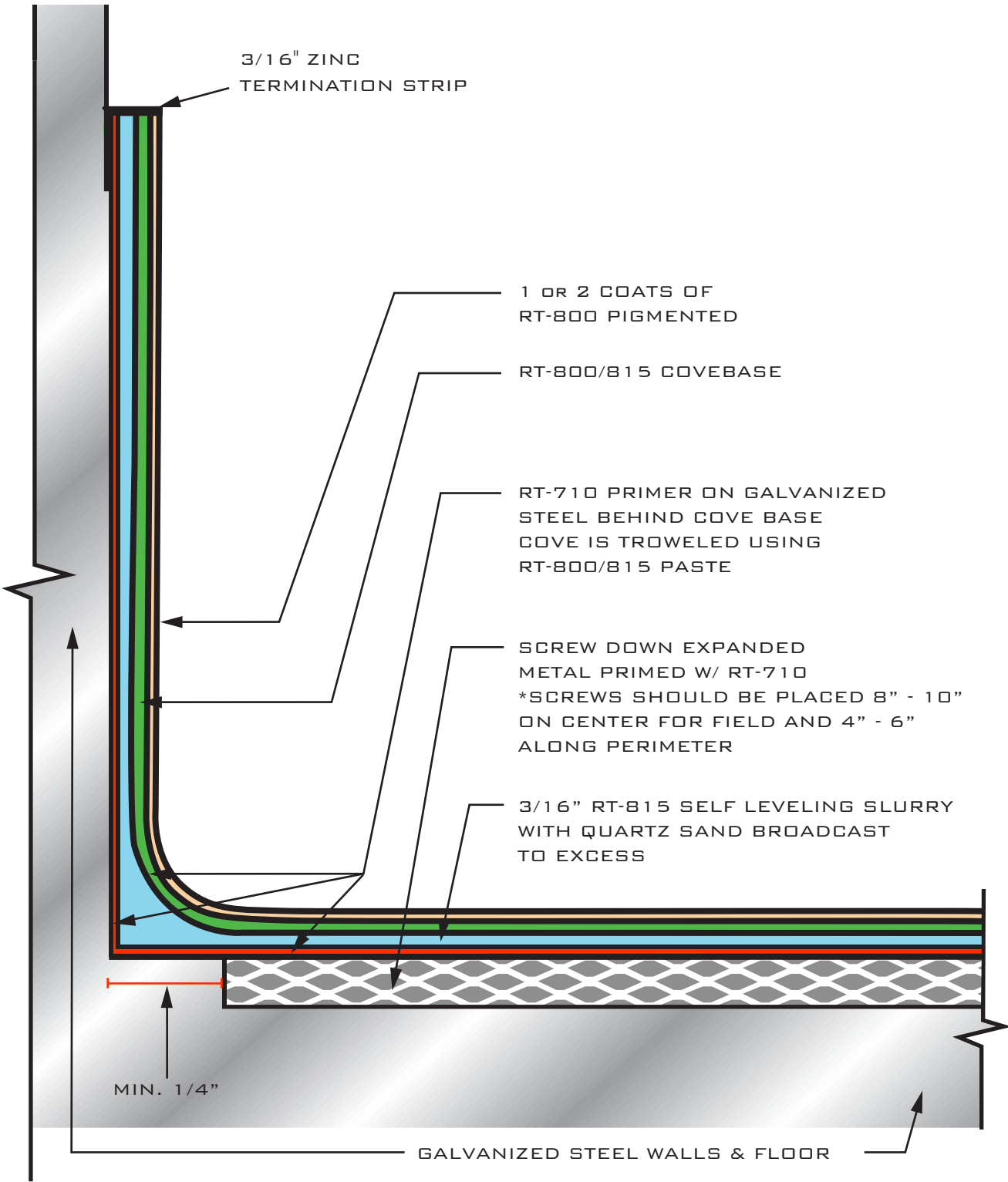
FIGURE F.2 FREEZER FLOORING SYSTEM NOT TO SCALE
