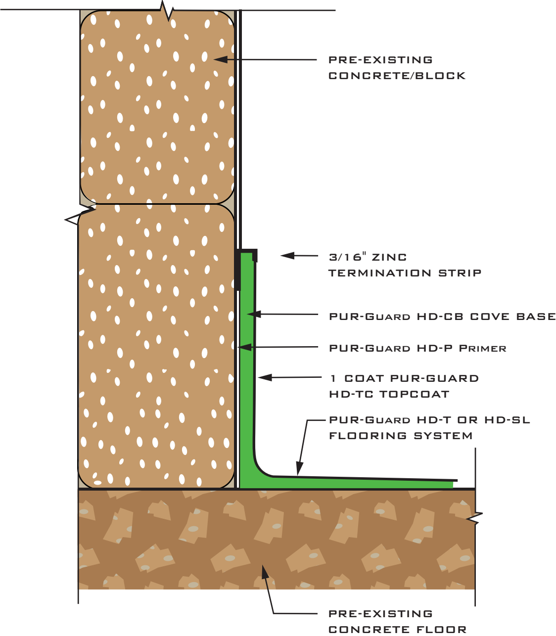
FIGURE PG.1 COVE BASE ON CONCRETE/BLOCK
